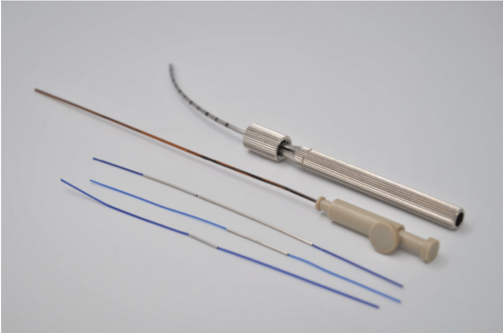
The Alpha DaRT Needle Applicator and components (18 gauge needle, 140 mm in length)
